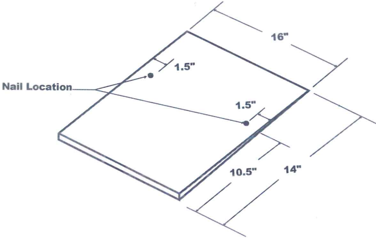
EAVE STARTER
