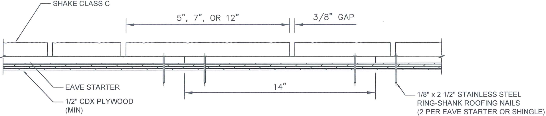
FRONT VIEW
